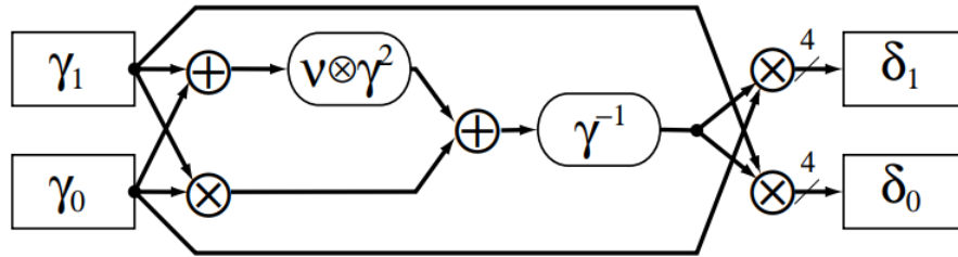
Figure 1: Normal GF(2^8) inverter: (\gamma_1 Y^{16} + \gamma_0 Y)^{-1} = (\delta_1 Y^{16} + \delta_0 Y) . The datapaths all have the same bit width (4 bits for this stage); addition is implemented via bitwise exclusive-OR, and sub-field multipliers are utilized. The GF(2^4) inverter follows the same recursive structure, while in GF(2^2) , inversion is computationally free, requiring only a bit swap.
